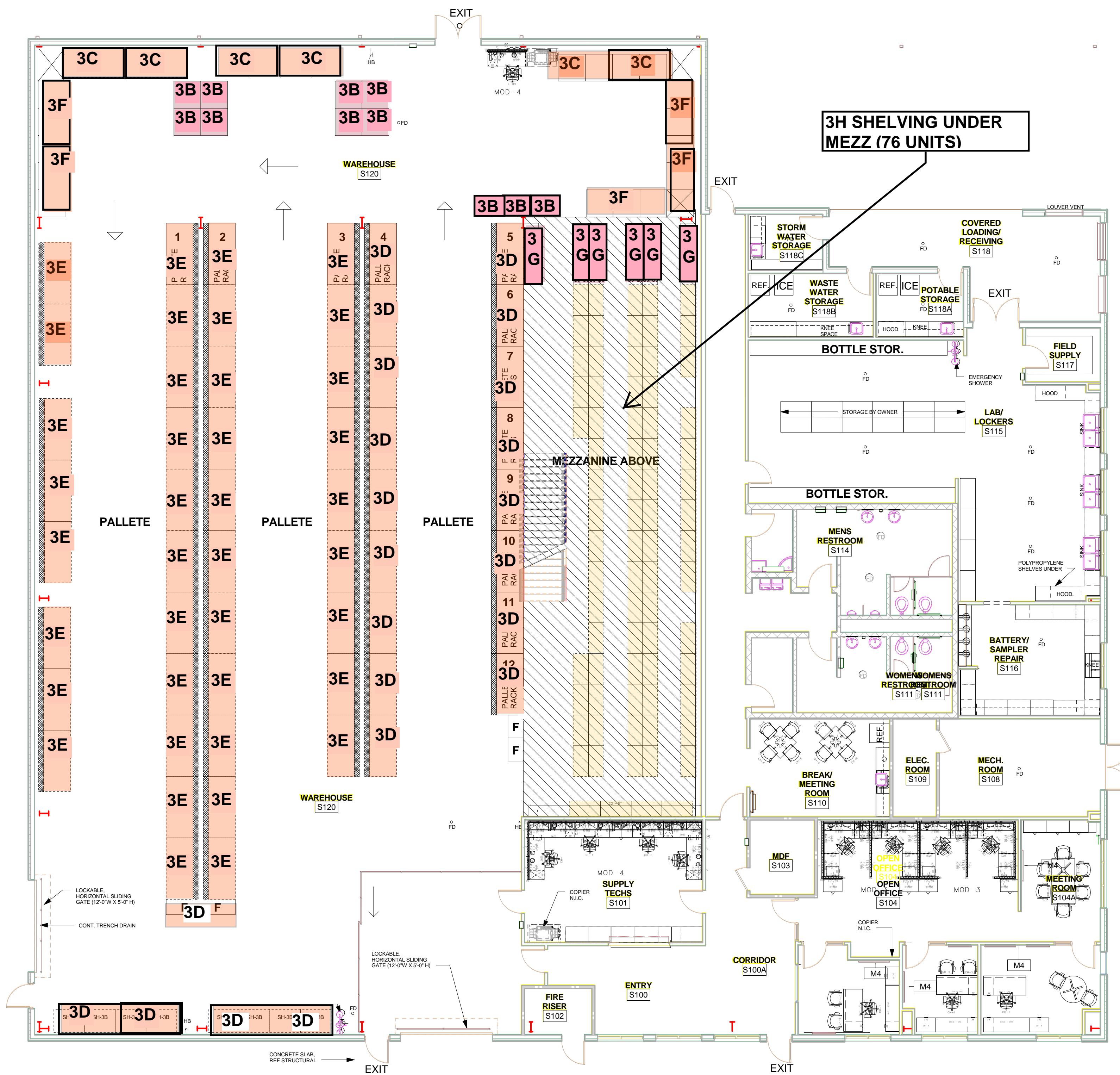
1 FURNITURE PLAN - SUPPLY BLDG LEVEL 1 1/8" = 1'-0"
